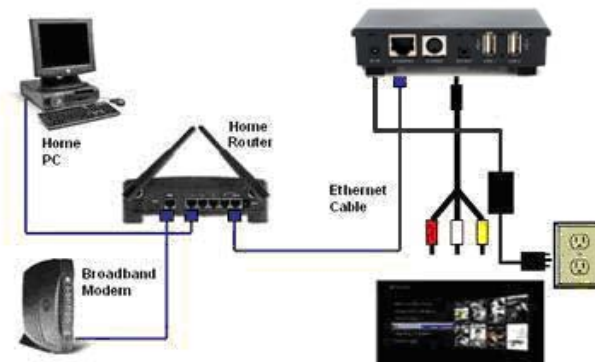
Figure 4 Connection using the Wired Ethernet
